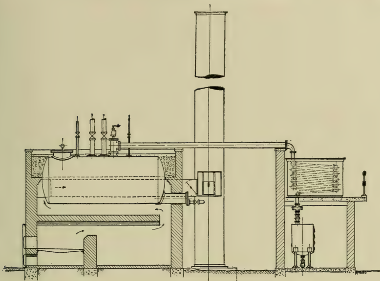
FIG. 97.—Horizontal Still for Refining Coal Tar.
